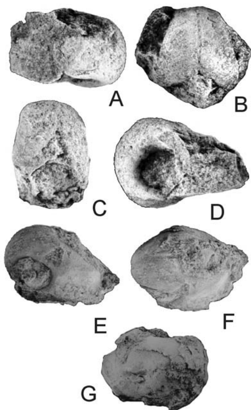
FIG. 1. A–D, Coelocyclus sp.; A, B, QMF37346 \times 2.3; C, D, QMF37347 \times 2.3; E–G, ? Tremanotus sp. QMF37342 \times 0.6.
